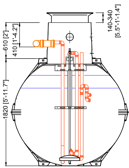
section SBR reactor
